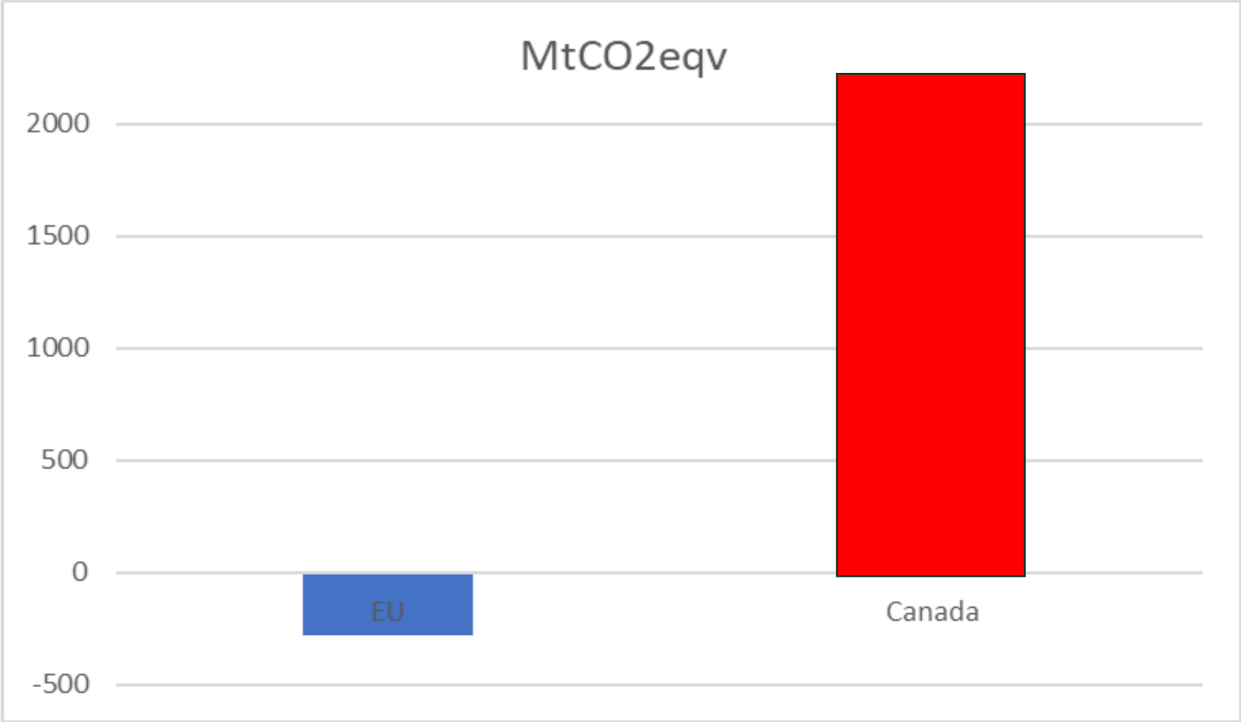
Byrne & al. 2024. Unprecedented Canadian forest fires carbon emissions 2023. (red bar)
